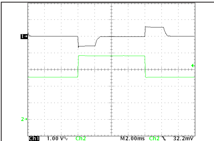
Figure 5: Output voltage response to step-change in load current (50%-75%-50% of I out (max); dI/dt = 0.1 A/μs). Load cap: 1 μF ceramic capacitor. Ch 1: V out , Ch 2: I out (2A/div).
