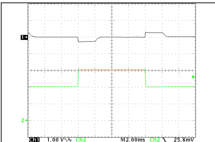
Figure 5: Output voltage response to step-change in load current (50%-75%-50% of I out (max); dI/dt = 0.1 A/μs). Load cap: 1 μF ceramic capacitor. Ch 1: V out , Ch 2: I out (5A/div).
