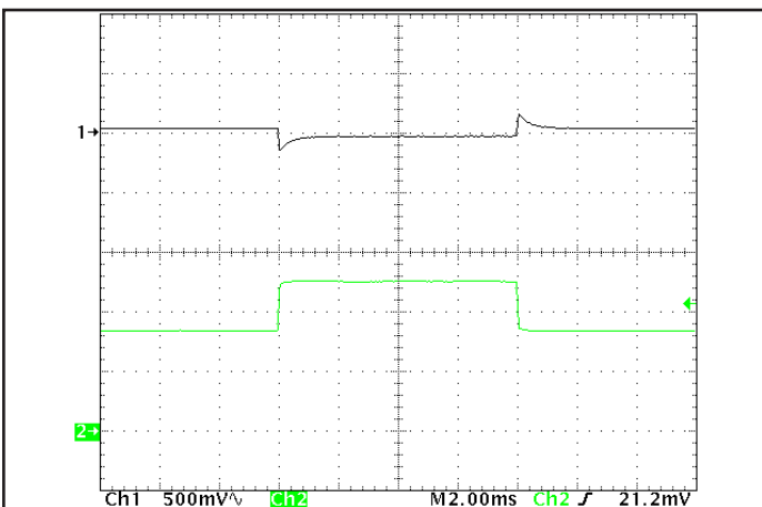
Figure 5: Output voltage response to step-change in load current (50%-75%-50% of I_{out(max)} ; dI/dt = 0.1 A/\mu s ). Load cap: 1 \mu F ceramic and 15 \mu F tantalum capacitors. Ch 1: Vout, Ch 2: I_{out} (25A/div)
